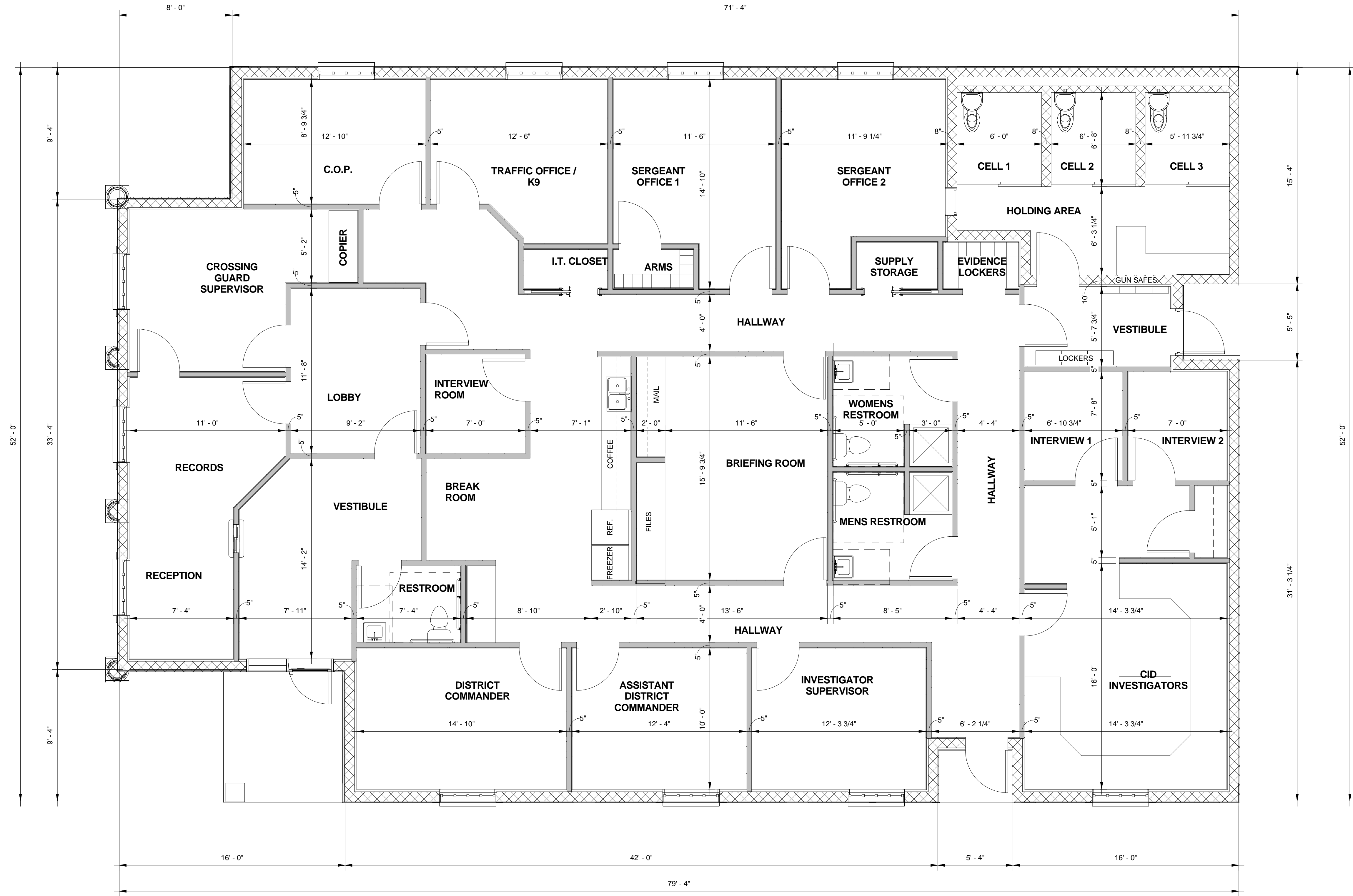
1 FLOOR PLAN 1/4" = 1'-0"
